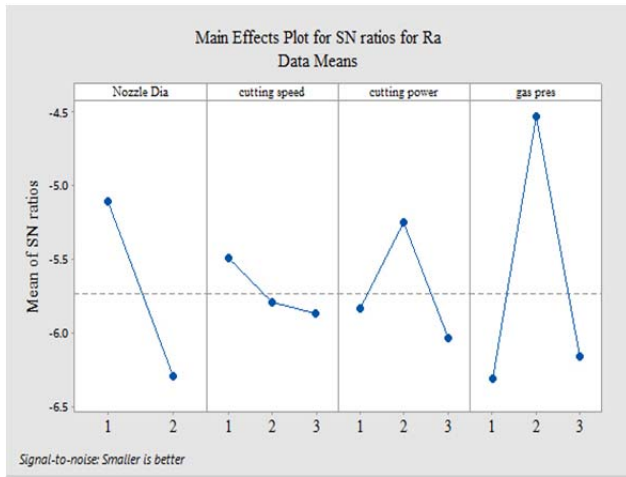
Fig. 1: Main effect plot for SR data S/N ratio
