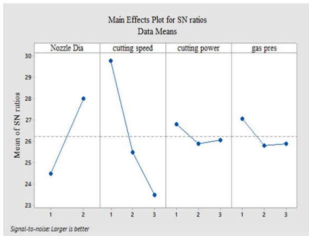
Fig. 2: Main effect plot for MRR data S/N ratio
